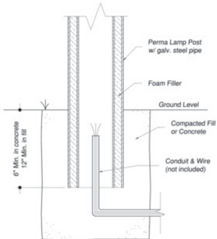
TYPICAL FOOTING SECTION FOR LAMP POST
