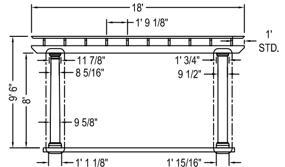
18' X 18' TRANQUILITY™ PERGOLA ROUND COLUMN OPTION
