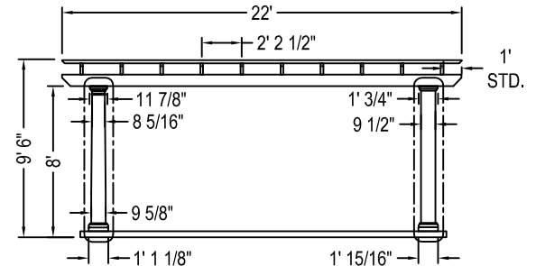
22' X 18' TRANQUILITY™ PERGOLA ROUND COLUMN OPTION
