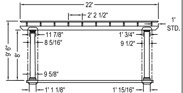
22' X 22' TRANQUILITY™ PERGOLA ROUND COLUMN OPTION 22' X 22' TRANQUILITY™ PERGOLA SQUARE COLUMN OPTION
