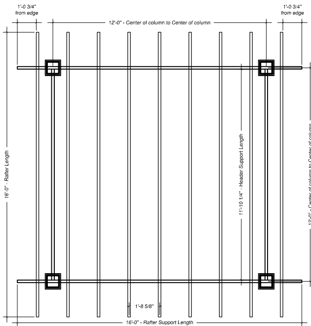
Rafters and Rafter Supports
