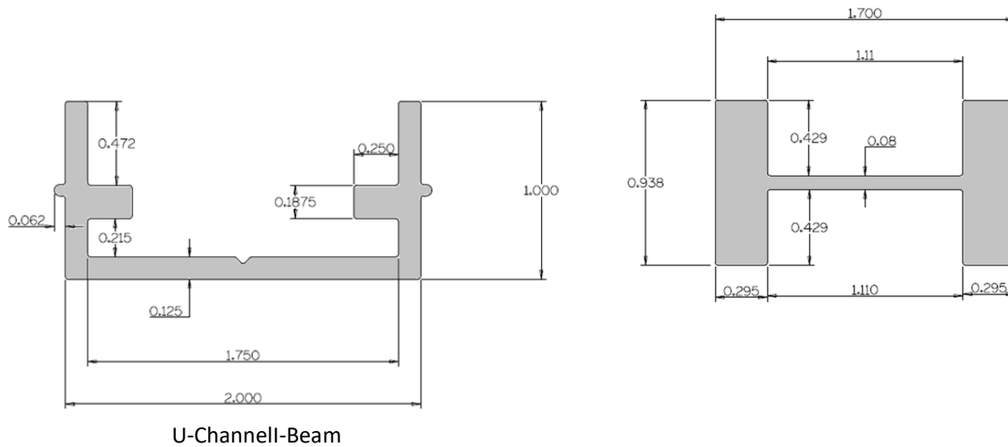
FIGURE 5 – ALUMINUM REINFORCEMENTS
