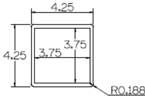
FIGURE 4 – 4.25" SQUARE NEWEL POST SLEEVE
