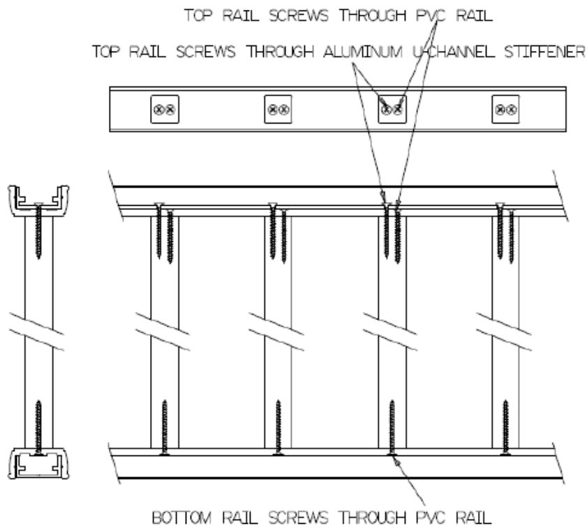
FIGURE 7 – INSTALLATION OF BALUSTERS
